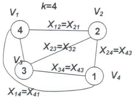
Fig. 1: Graph coloring example
