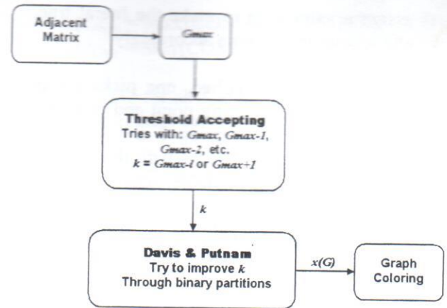
Fig. 2: Description of the coloring process.
