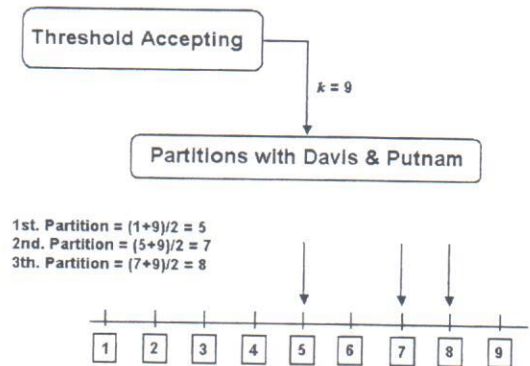
Fig. 3: Binary partitions.
