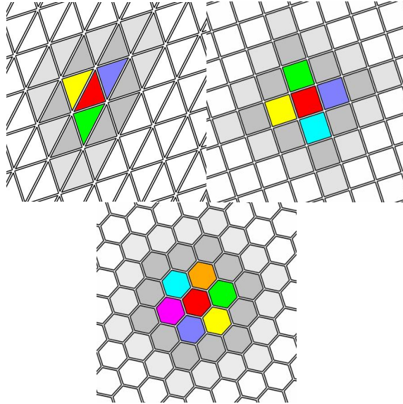
Fig. 1. The entropy of triangular (a), square (b) and hexagonal (c) cell shapes. The number of neighbors is marked with different colors to the given red cell in the middle.
