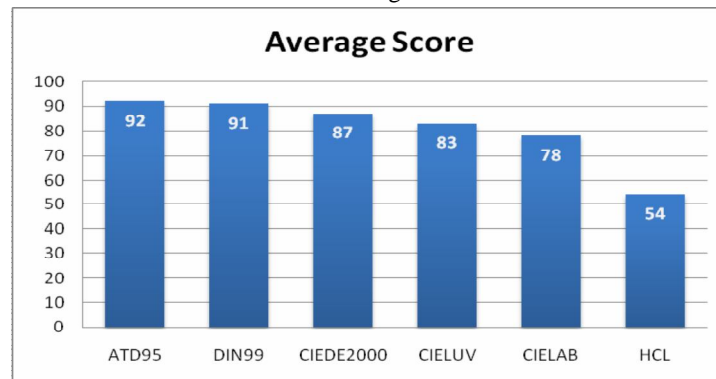
Fig. 3. Average score for the different color metrics using the experimental image set 1 as judged by 10 human observers.
